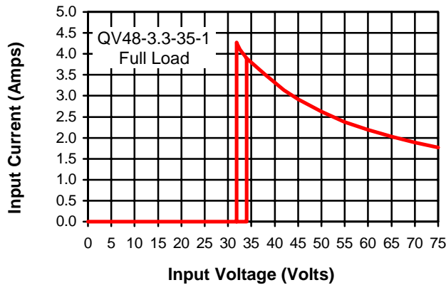
Input Characteristics
