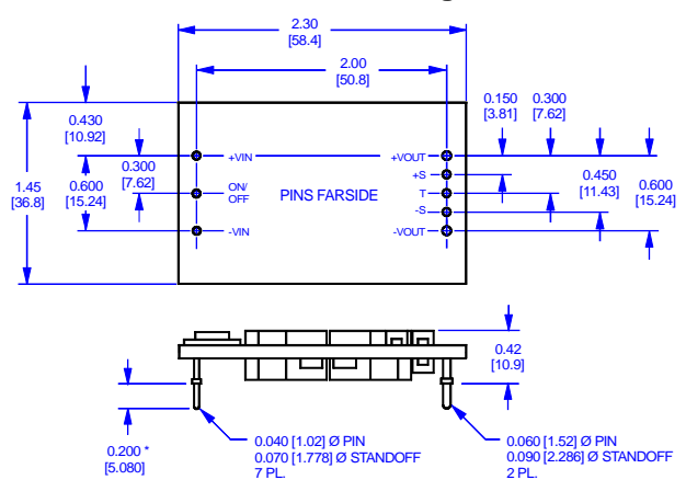
Outline Drawing
