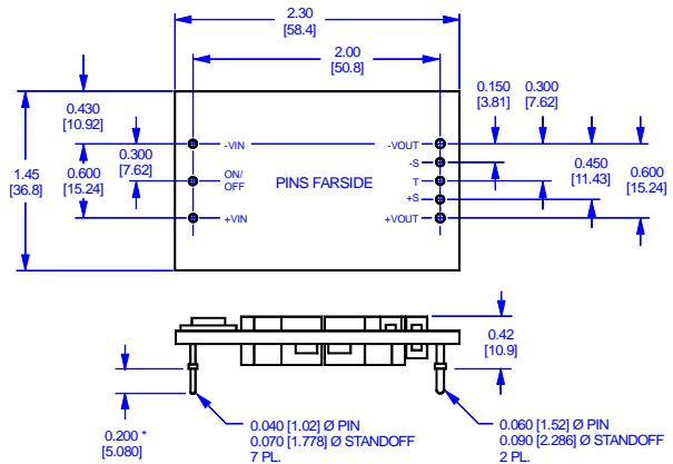
Outline Drawing
