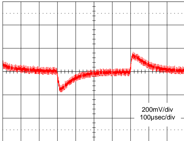
Transient Response
