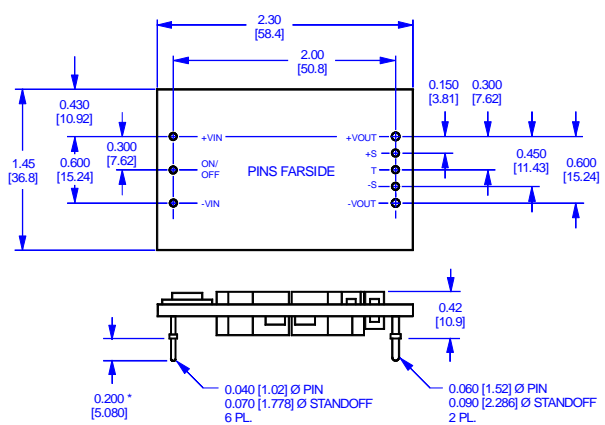
Outline Drawing
