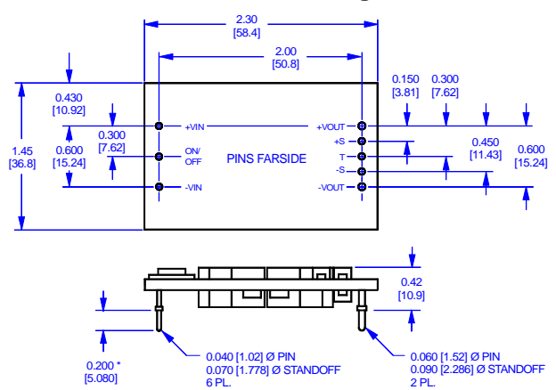
Outline Drawing
